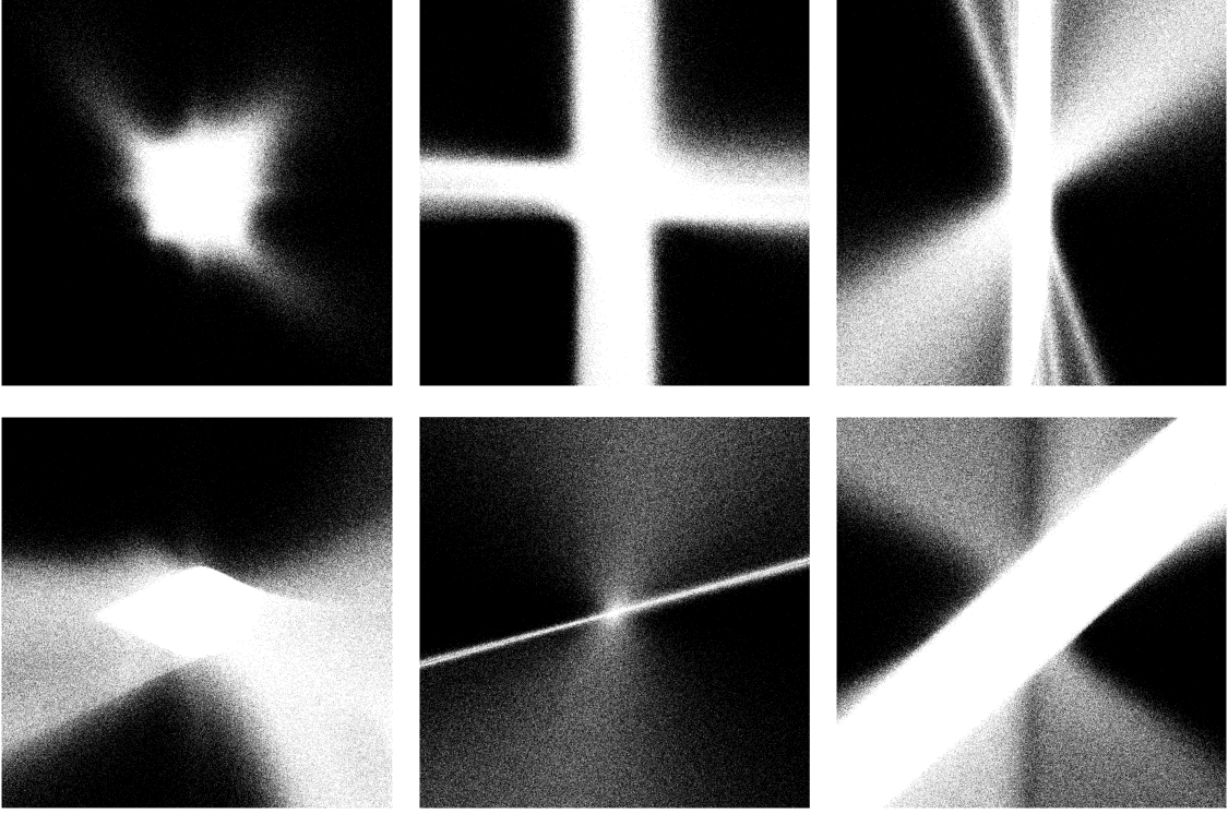
Figure 1: Gallery of convergence landscapes. Top left is generated with seed 1 and W_K = W_Q = I . The rest are generated with random seeds (from left to right, top to bottom): 1679700, 5227590, 6306593, 6549664, and 8012376. The corresponding weight matrices for each seed are provided in Appendix B.
